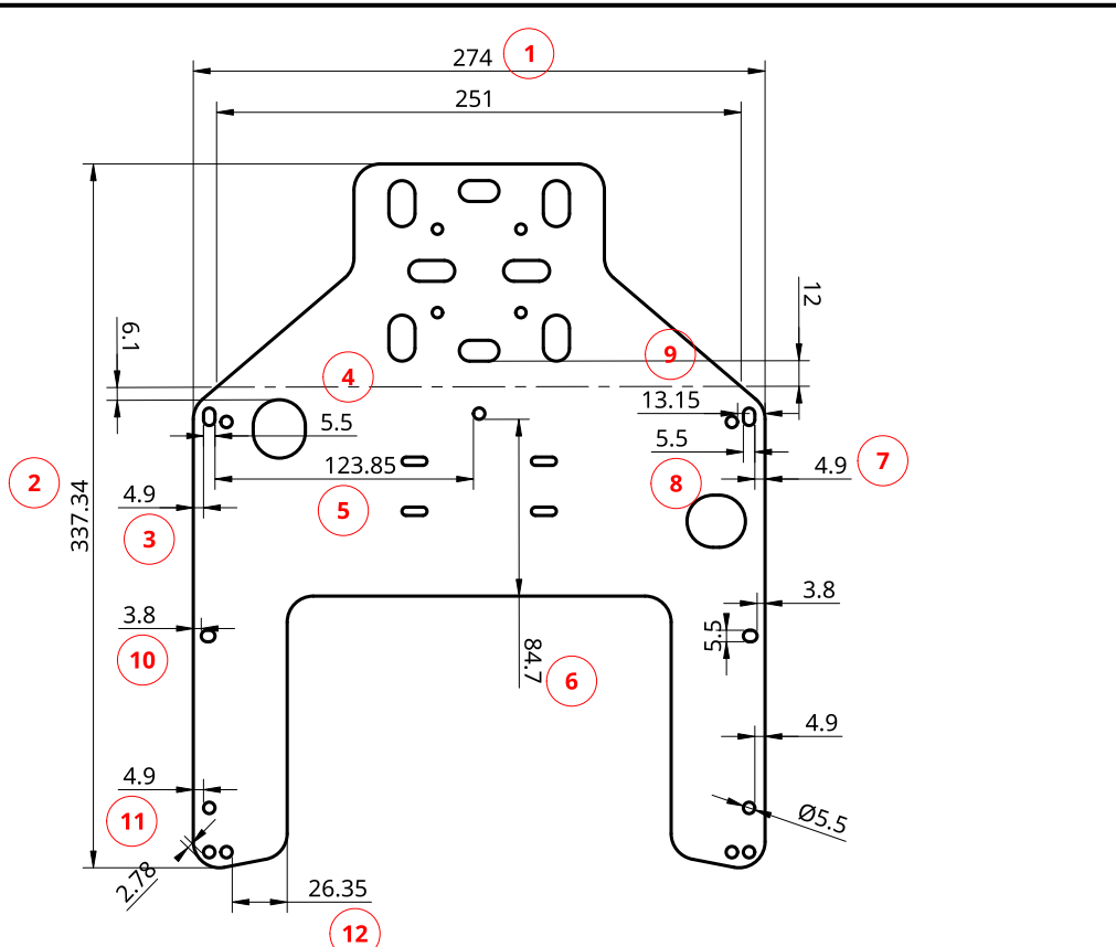
Flat Dimensions
